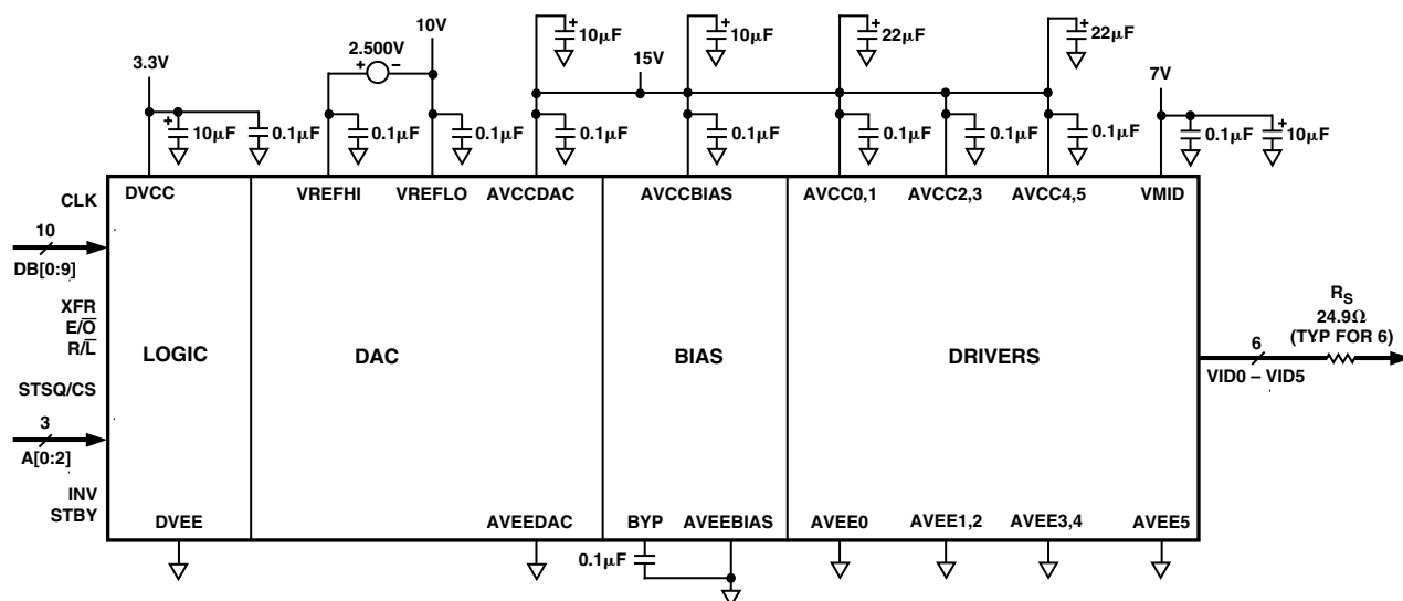
Figure 10. Interface Drawing
