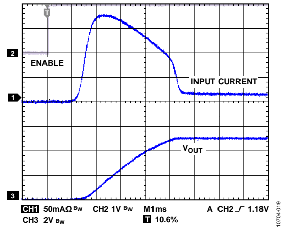
Figure 20. Typical Turn-On Time and Inrush Current, V_{IN} = 5\text{ V} , C_{OUT} = 100\ \mu\text{F} , 330\ \Omega Load
