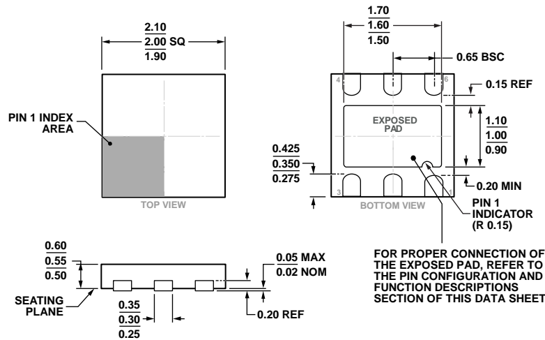
Figure 29. 6-Lead Lead Frame Chip Scale Package [LFCSP_UD] 2.00 mm x 2.00 mm Body, Ultra Thin, Dual Lead (CP-6-3) Dimensions shown in millimeters
