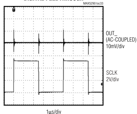
DIGITAL FEEDTHROUGH
