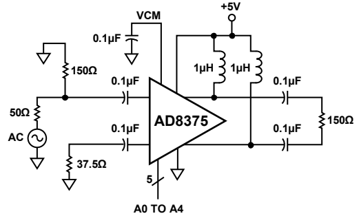
Figure 33. Single-Ended-to-Differential Conversion
