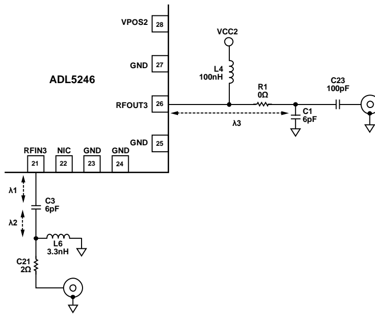
Figure 76. AMP3 Matching Circuit at 0.9 GHz
