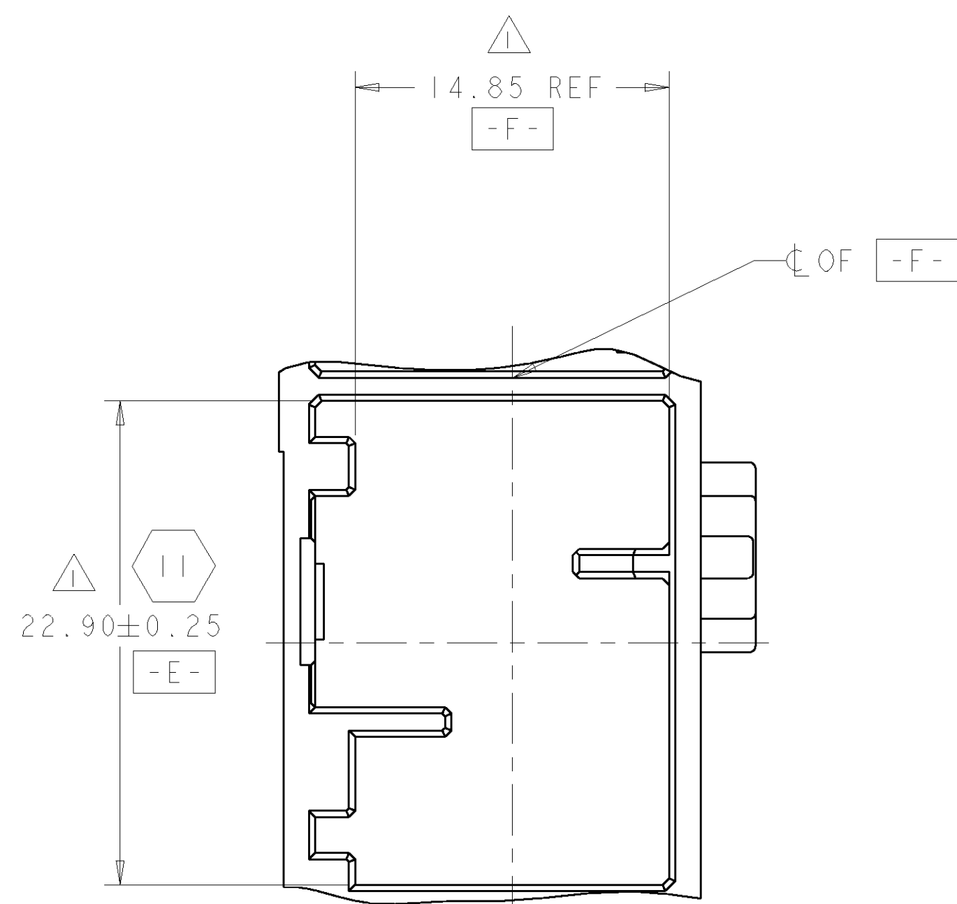
DETAIL XX SCALE 4:1
