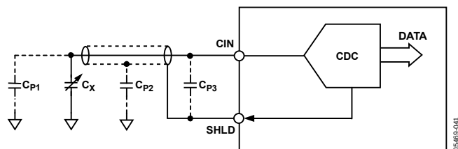
Figure 33. Parasitic Capacitance
