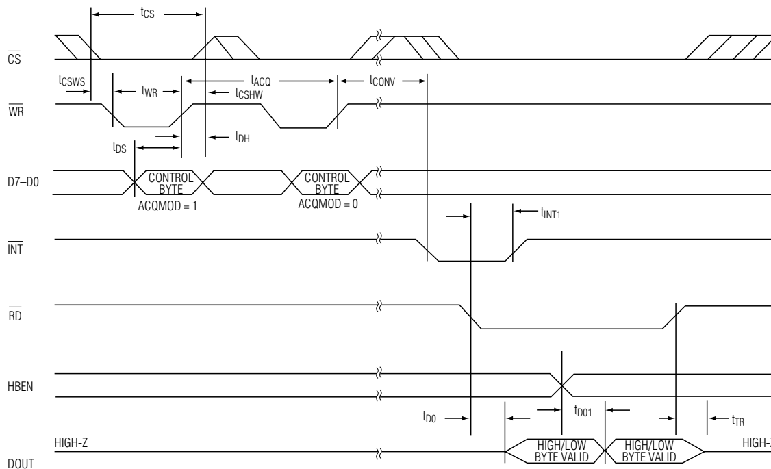
Figure 5. Conversion Timing Using External Acquisition Mode
