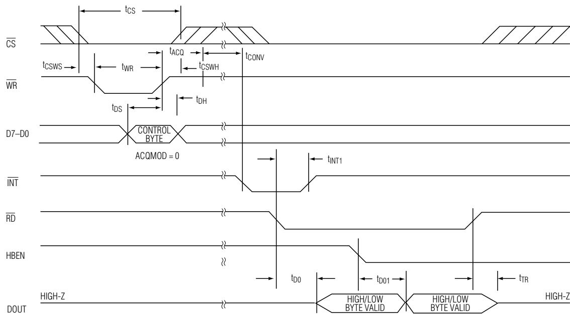
Figure 4. Conversion Timing Using Internal Acquisition Mode
