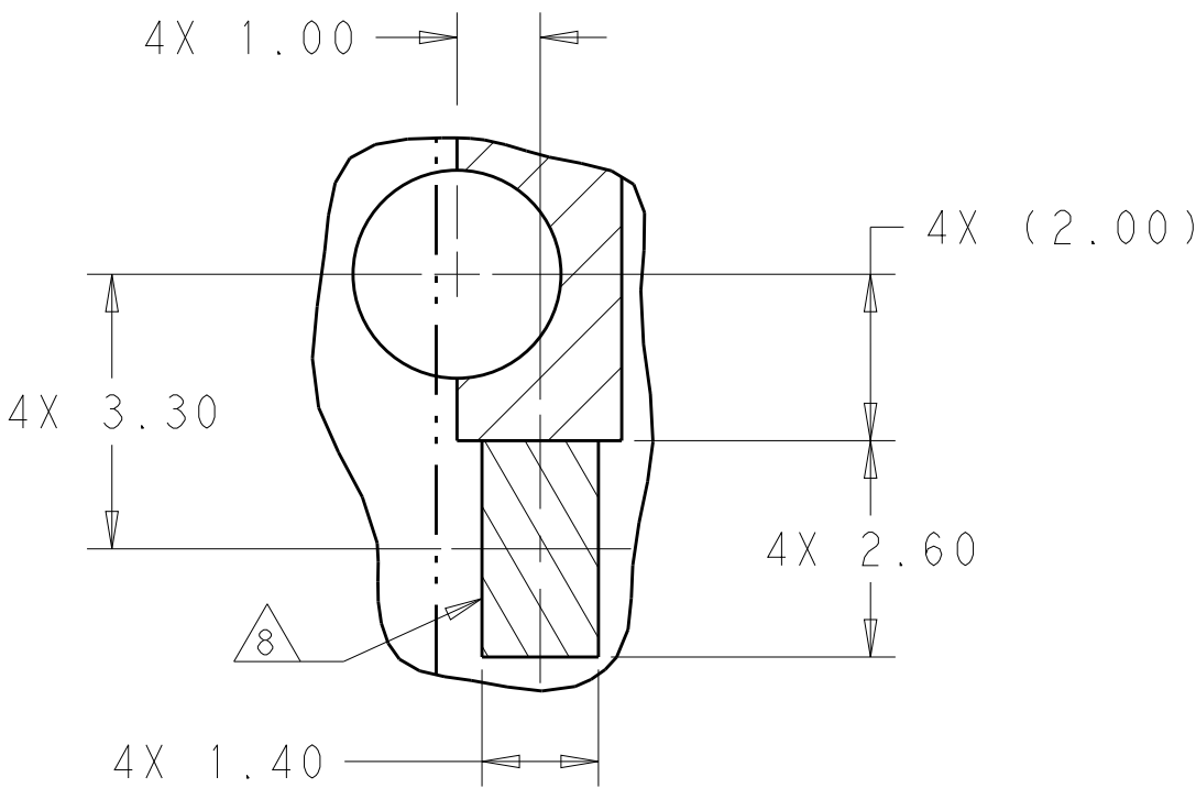
DETAIL J LED PADS SCALE 10:1
