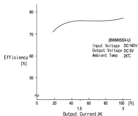
Efficiency Curve
