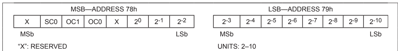
Figure 9. RSGAIN Register
