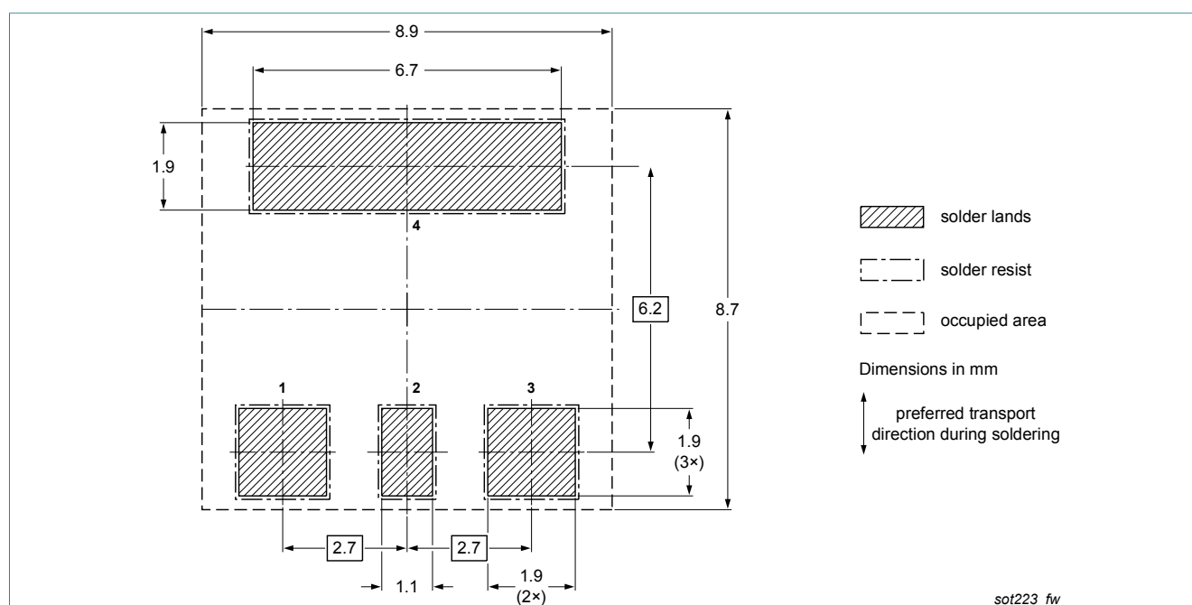
Fig. 19. Wave soldering footprint for SOT223 (SC-73)
