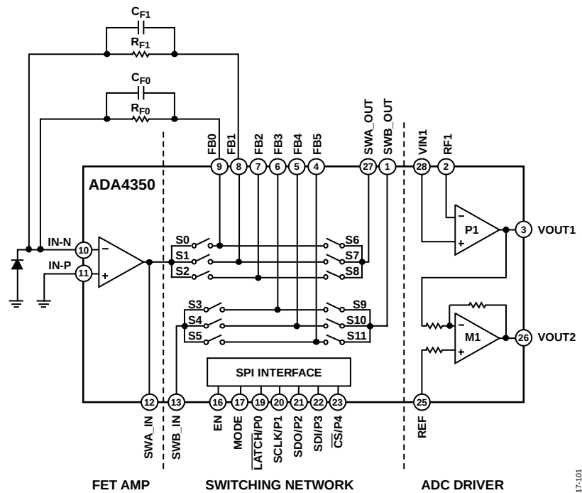
Figure 55. Simplified Schematic
