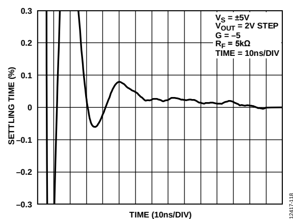
Figure 20. 0.1% Settling Time
