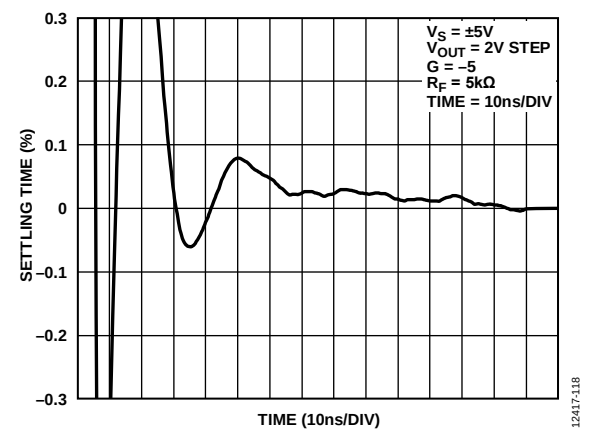
Figure 20. 0.1% Settling Time
