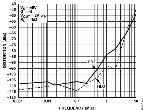
Figure 21. Distortion (HD2/HD3) vs. Frequency, G = -5
