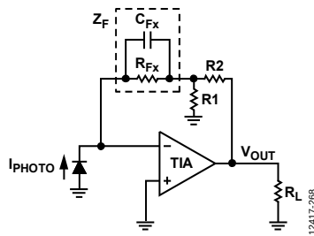
Figure 70. T Network
