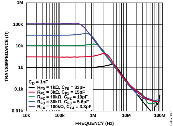
Figure 63. Transimpedance vs. Frequency, C_D = 1 nF
