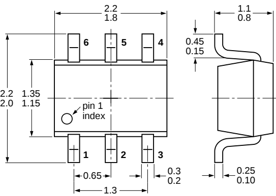
Fig 11. Package outline PUMH18 (SOT363)
