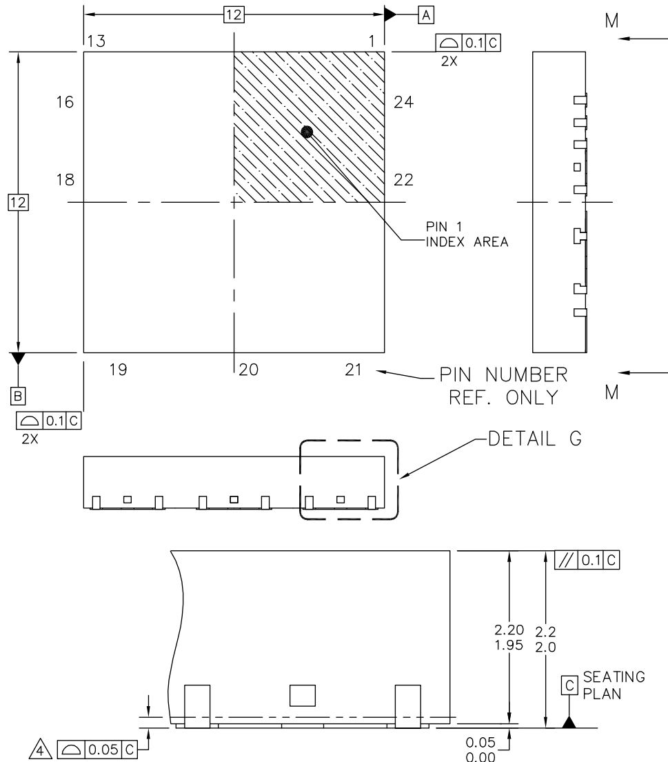
DETAIL G
