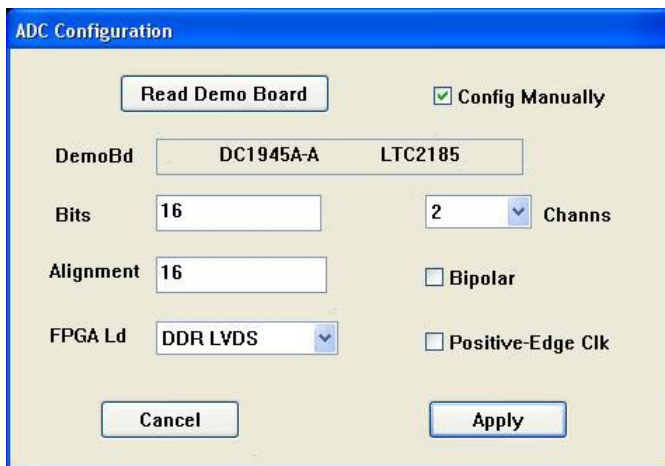
Figure 2. ADC Configuration
