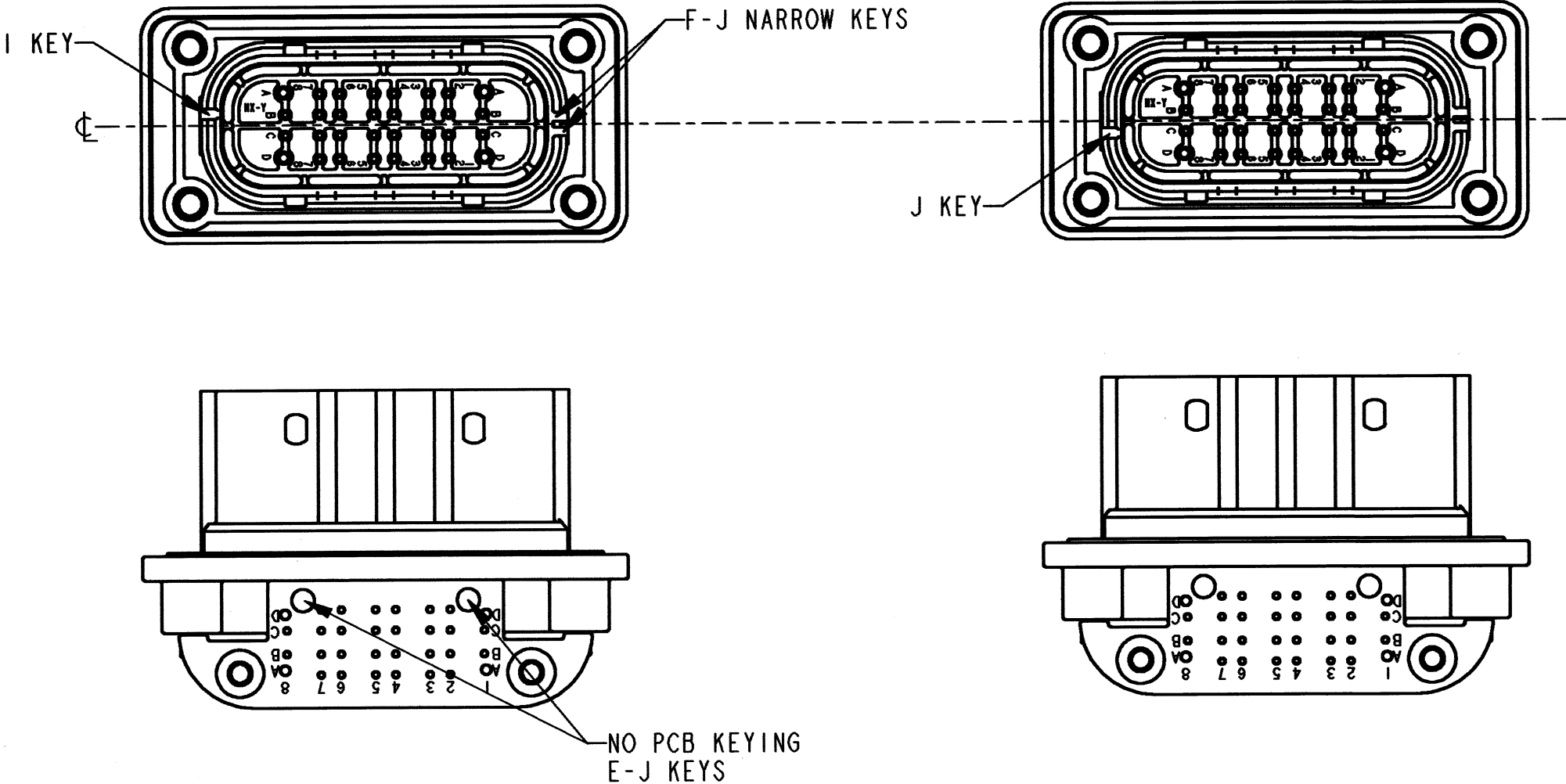
KEY ARRANGEMENT -I- SRK13-MDI-32A-001
