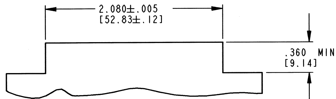
PC BOARD
