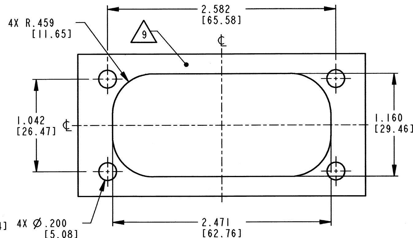
PANEL CUTOUT
