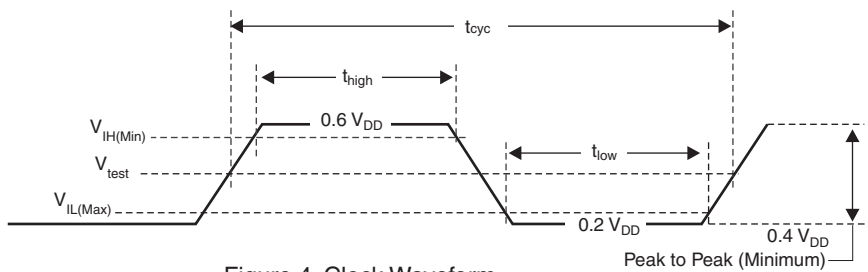
Figure 4. Clock Waveform
