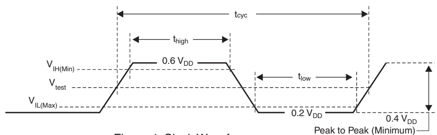
Figure 4. Clock Waveform
