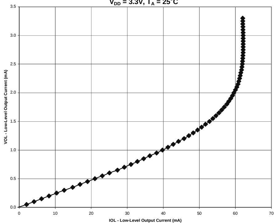
ICS9112AG-27 LOW-LEVEL OUTPUT VOLTAGE vs LOW-LEVEL OUTPUT CURRENT V_{DD} = 3.3V, T_A = 25^{\circ}C
