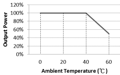
OUTPUT POWER DERATING CURVE
