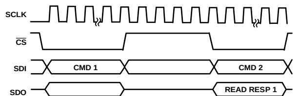
Figure 53. Off Frame Protocol
