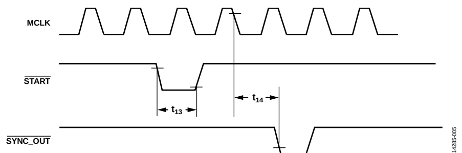
Figure 5. Asynchronous \overline{\text{START}} and \text{SYNC\_OUT} Timing Diagram
