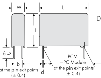
4-pin version
