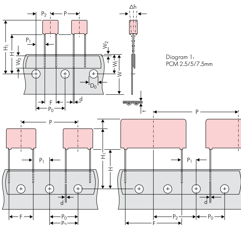
Diagram 2: PCM 10/15 mm
