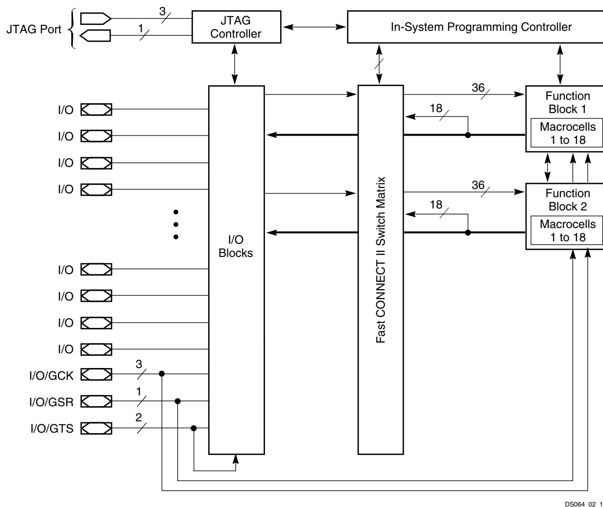
Figure 2: XC9536 Architecture
