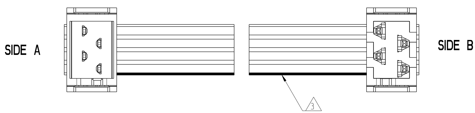
2205112-X (4 POSITION CABLE ASSEMBLY) AS SHOWN
