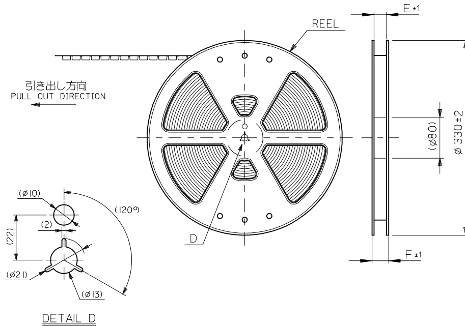
DETAIL D
