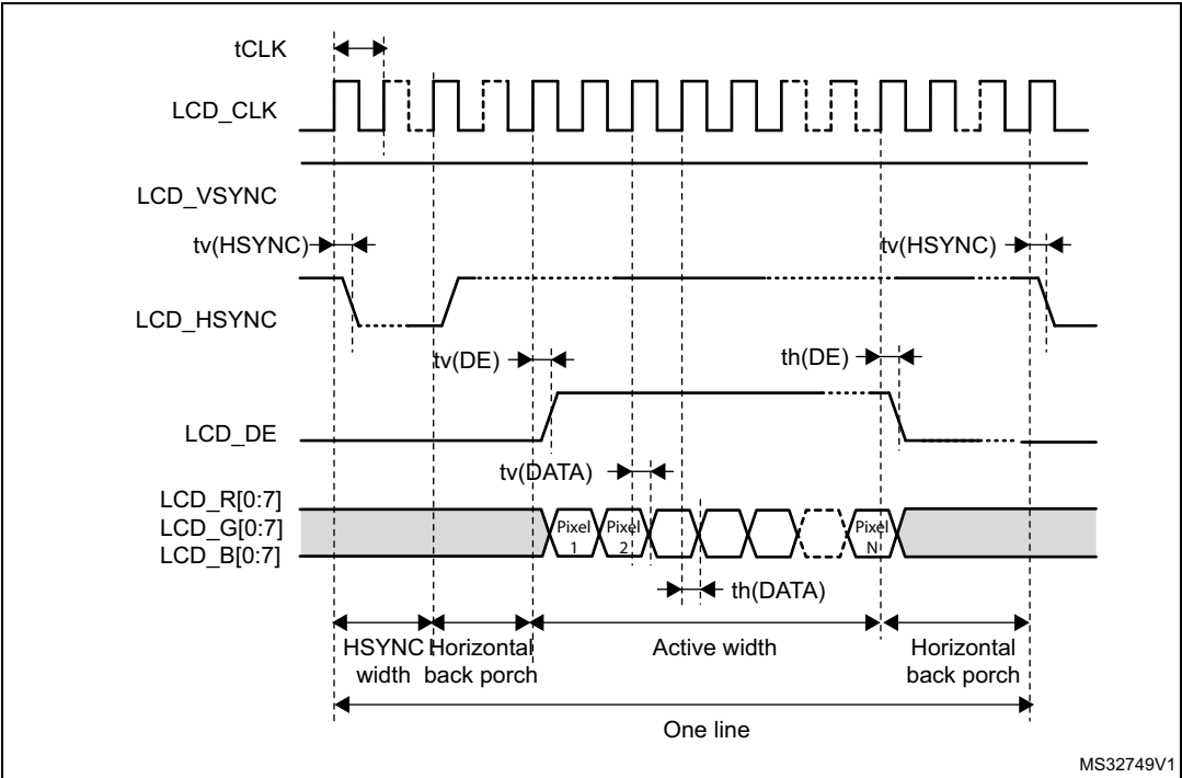
Figure 79. LCD-TFT horizontal timing diagram
