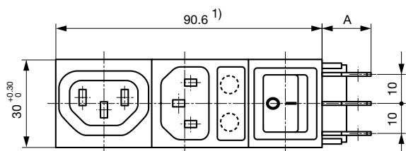
Variants 6432.0X5X.XX Mounting hole: 90.6+0,2 \times 27.6+0,2 A: Quick-connect terminal 6.3 \times 0.8 mm: 18.1 mm A: Solder terminal 3.5 \times 0.8 mm: 13.3 mm S: Panel thickness
