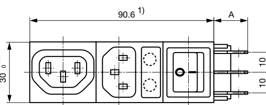
Variants 6432.0X5X.XX Mounting hole: 90.6+0,2 x 27.6+0,2 A: Quick-connect terminal 6.3x0.8 mm: 18.1 mm A: Solder terminal 3.5x0.8 mm: 13.3 mm S: Panel thickness
