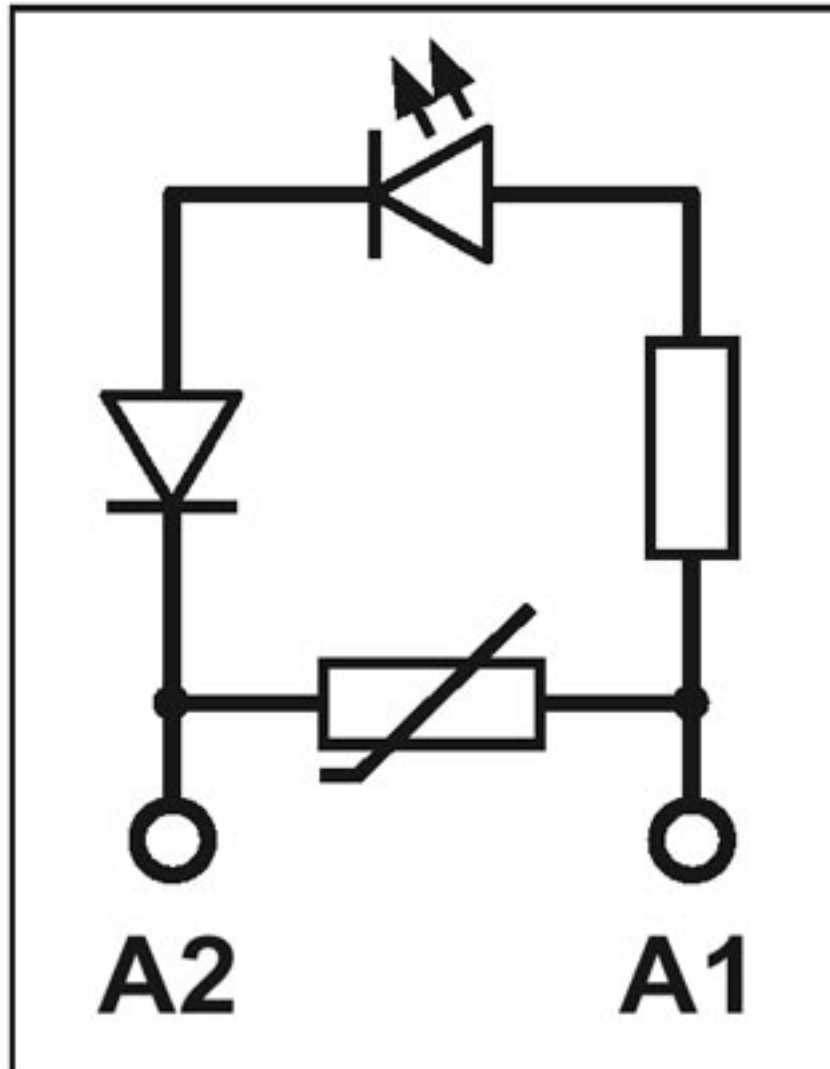
Circuit diagram
