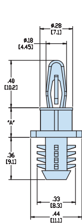
BAYONET SNAP LOCK 10,2 / BLIND FIR TREE
