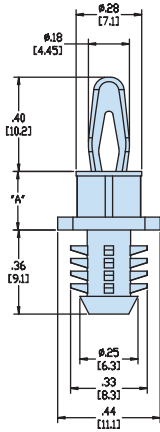
BAYONET SNAP FIT 10,2 / BLIND FIR TREE
