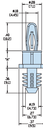
BAYONET SNAP LOCK 10,2 / BLIND FIR TREE
