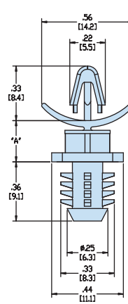
ARROWHEAD SNAP LOCK / BLIND FIR TREE
