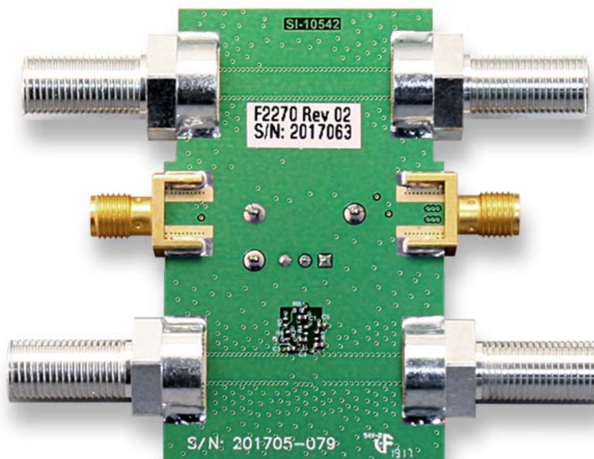
Figure 59. Evaluation Kit Bottom View
