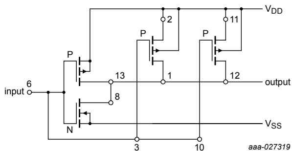
Figure 13. High current source driver
