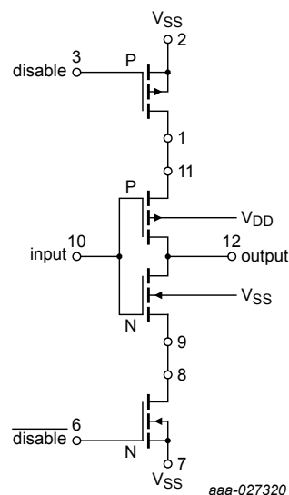
Figure 14. High impedance buffer
