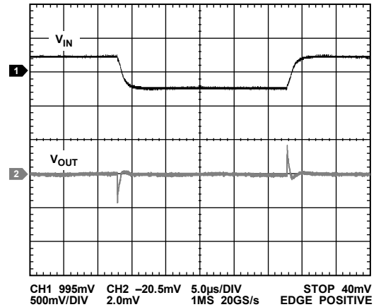
Figure 37. Line Transient Response, 500 mV Step, V_{OUT} = -3.3 V , I_{LOAD} = -500 mA
