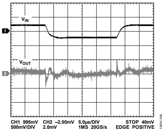
Figure 36. Line Transient Response, 500 mV Step, V_{OUT} = -1.2 V , I_{LOAD} = -500 mA
