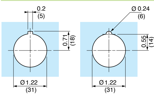
Preferred Cut-Out Alternate Cut-Out Use Greenlee Tool #60242 for punching hole and notch.
