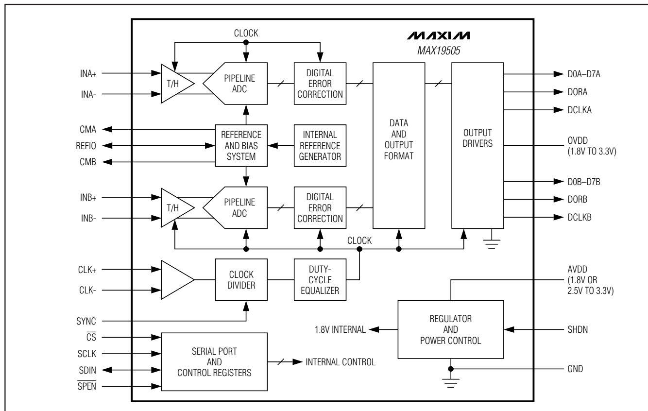
Figure 2. Functional Diagram
