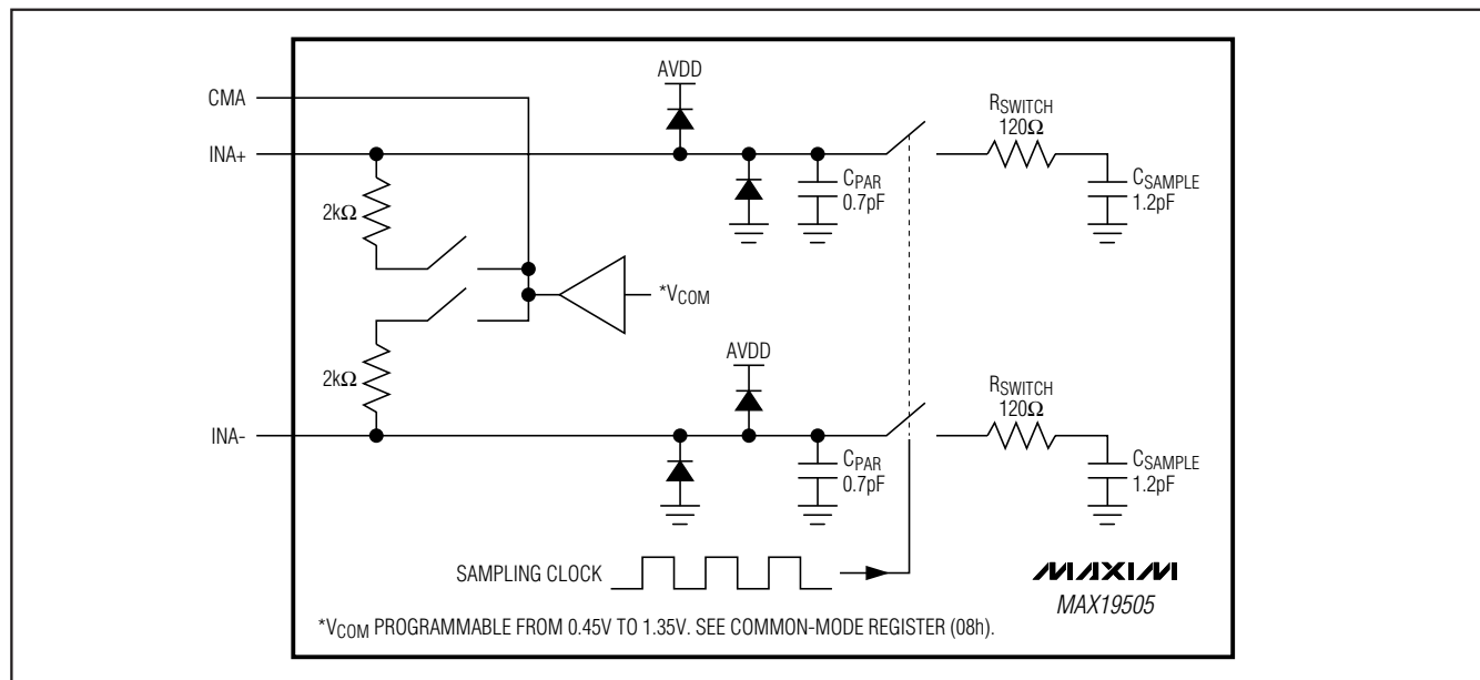
Figure 3. Internal Track-and-Hold (T/H) Circuit
