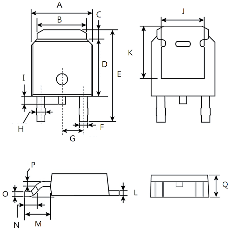
TO-252 (D-PAK)
