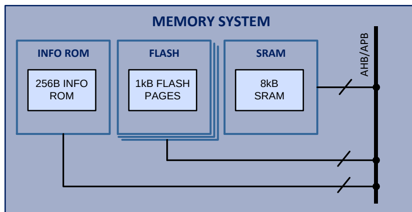
Figure 15-1 Memory System
