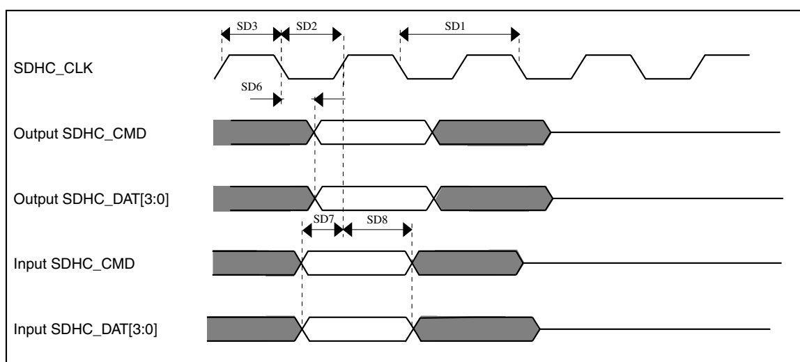
Figure 34. SDHC timing
