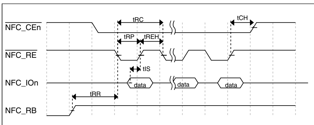
Figure 15. Read data latch cycle timing in Slow mode
