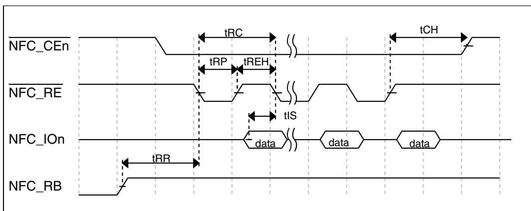
Figure 16. Read data latch cycle timing in Fast mode and EDO mode
