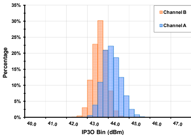
IP 30 Distribution ( F_{RF} = 1850\text{MHz} , LC mode, N = 3168 )
