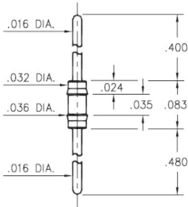
8006-0-00-XX-00-00-03-0 Press-fit in .034 mounting hole
