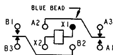
TERMINAL VIEW
