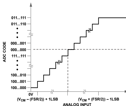
Figure 25. Twos Complement Transfer Function
