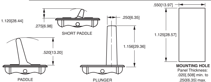
TERMINAL TYPE
