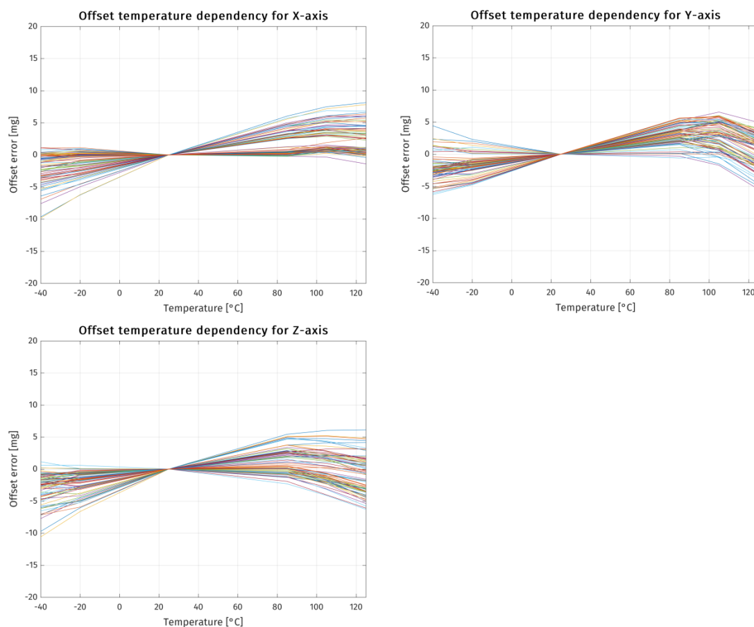
Figure 2. SCA3300-D01 accelerometer typical offset temperature behavior.
