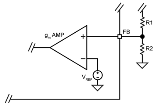
Figure 7. Voltage-Divider Configuration
