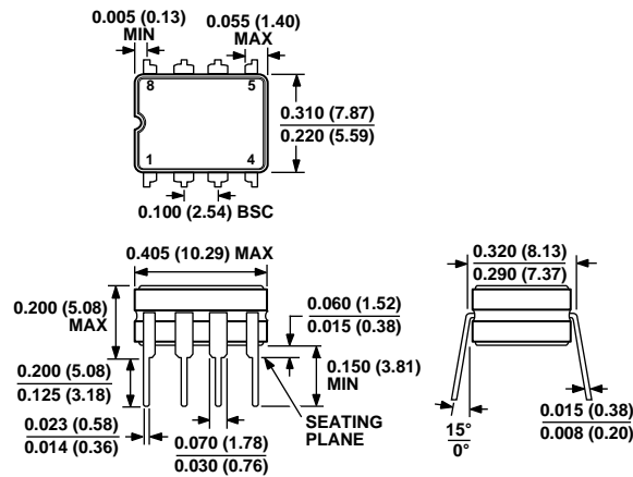
Figure 64. 8-Lead Plastic Dual In-Line Package [PDIP] Narrow Body (N-8) Dimensions shown in inches and (millimeters)
