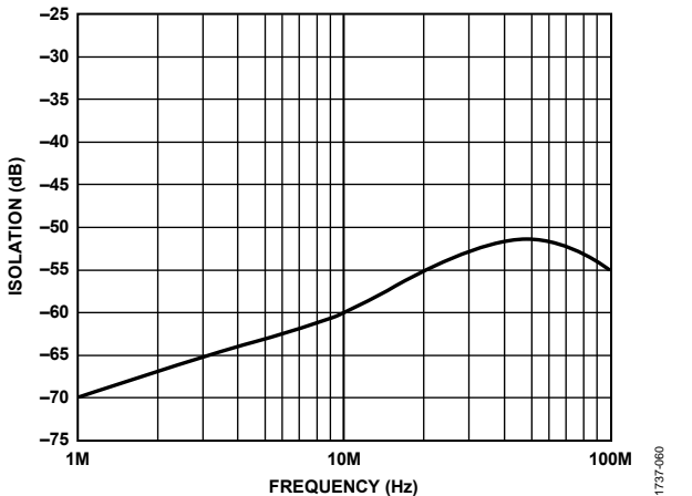
Figure 62. Isolation vs. Frequency for 4:1 Mux, Off Channel
